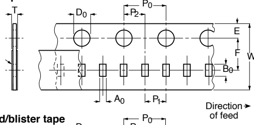
Embossed/blister tape
